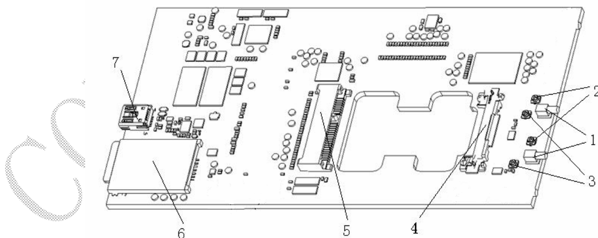
Figure 5-10 Structure of the debugging board
