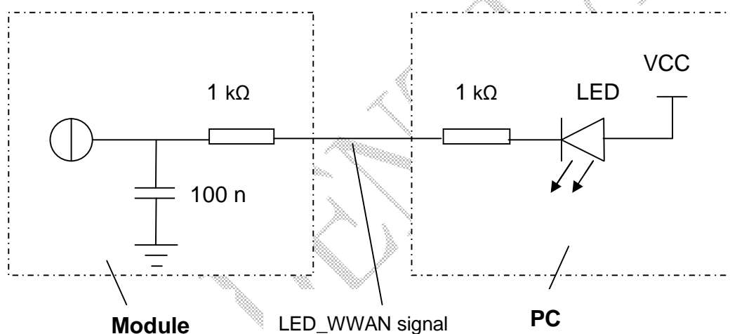
Figure 3-2 LED_WWAN# signal reference circuit diagram
