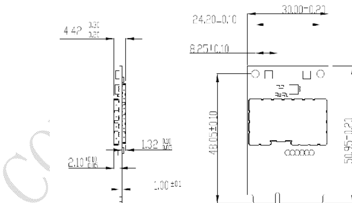
Figure 2-1 Dimensions of the EM660C
