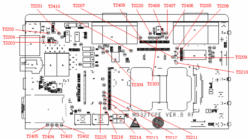
Figure 5-13 Test point position
