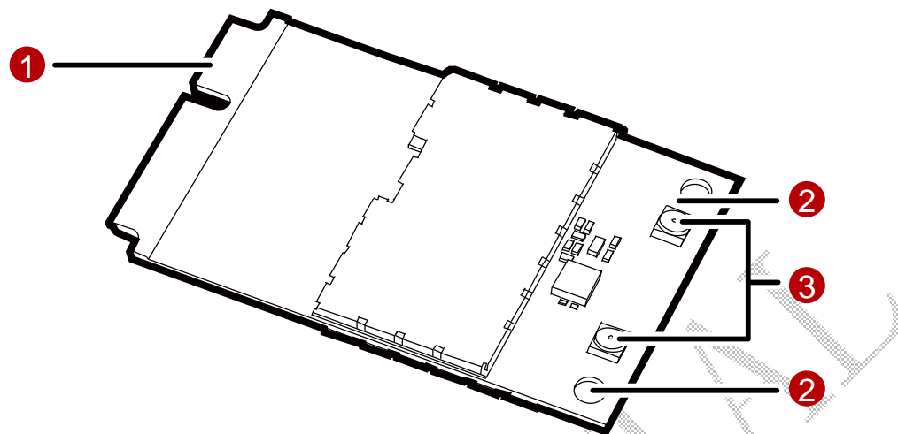
Figure 2-2 Appearance of the interfaces on the EM660C
