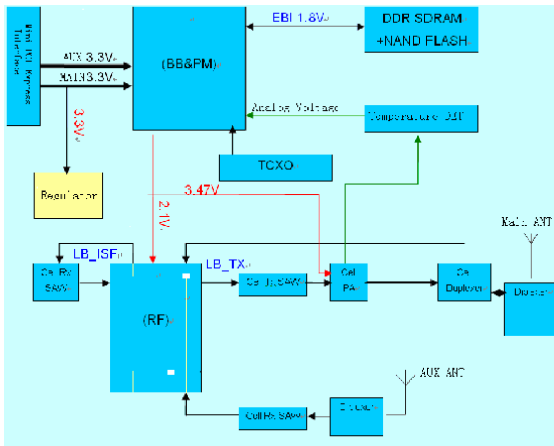
Figure 1-2 Hardware functional block diagram
