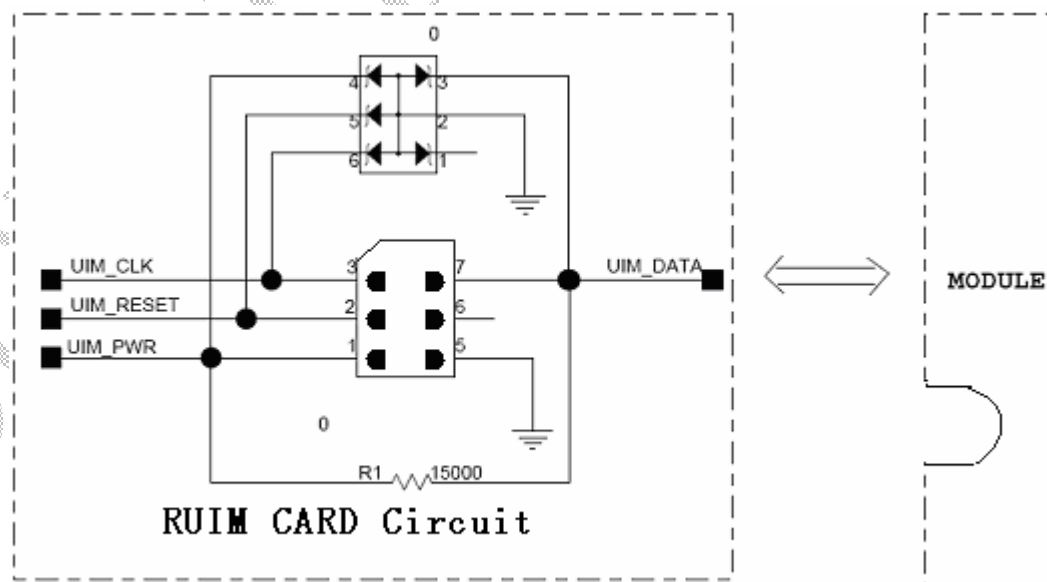
Figure 3-1 RUM interface schematic on user's PC
