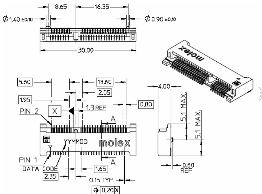
Figure 2-3 Dimensions of the Mini PCI Express connector
